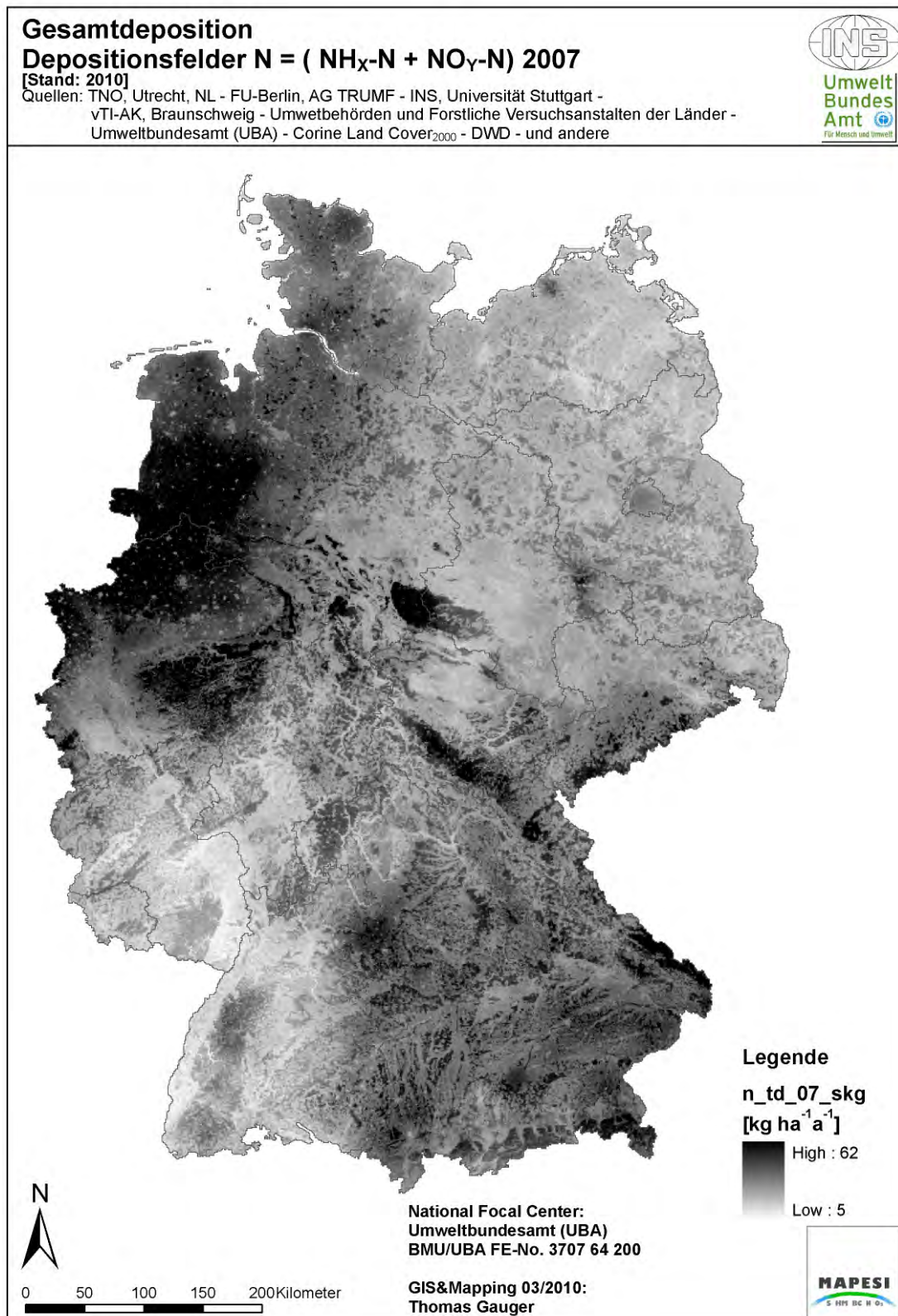
Abb. A.I.6: Gesamtdeposition von Stickstoff 2007 [kg ha -1 a -1 ] Quelle: Builtjes et al., 2011 [30]
